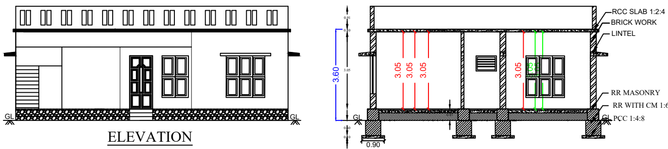
SECTION X-X'
