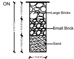
SECTION OF RAIN WATER COLLECTION PITS (NTS)
