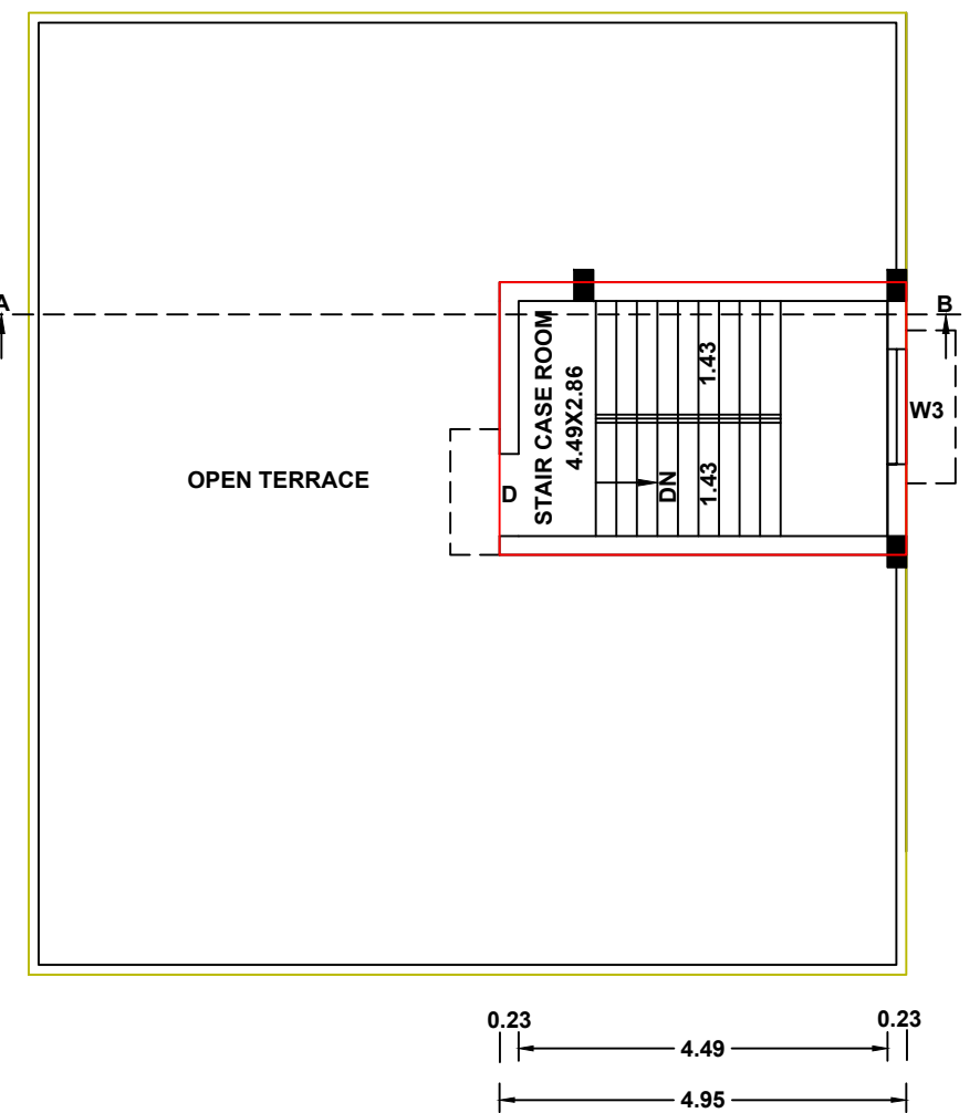
HEAD ROOM PLAN (Scale 1:100)
