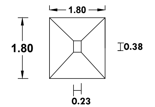
SECTION OF COLUMN
