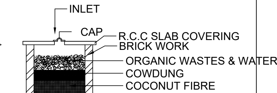
COMPOST PIT - SECTION
