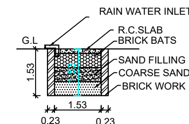
RAIN WATER HARVESTING TANK RWH_CAPACITY_L=5000LTRS
