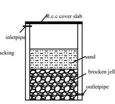
Section of Rainwatertank
