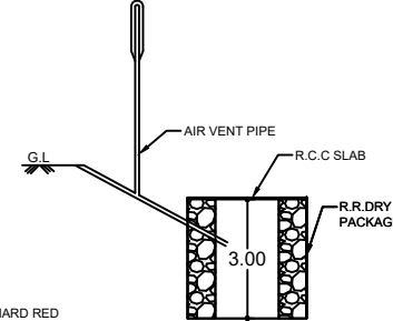
SECTION OF SOAKPIT
