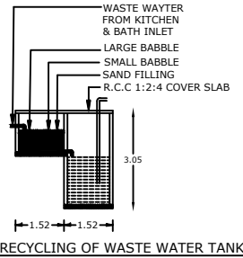
RECYCLING OF WASTE WATER TANK
