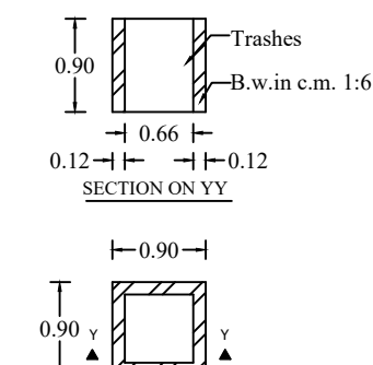
WASTE TRASH PIT
