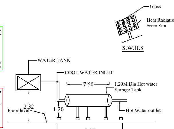
SOLAR WATER HEATING SYSTEM ( S.W.H.S.DETAILS)
