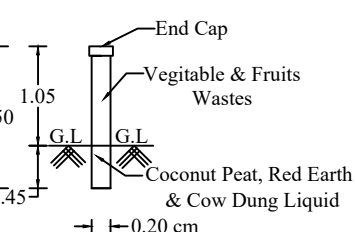
PIPE COMPOSTER
