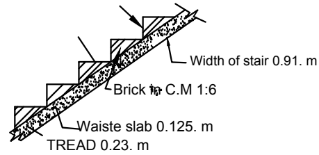
Stair Details
