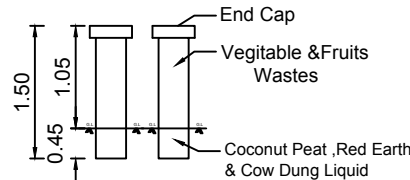
PIPE COMPOSTER
