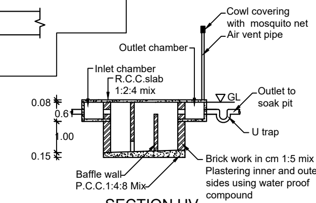
SECTION UV
