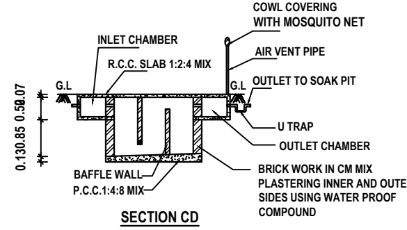
SECTION CD
