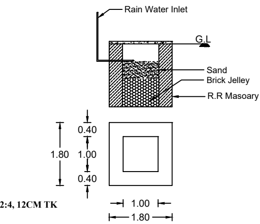
RAIN WATER HARVESTING DETAILS
