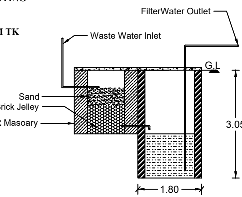
RECYCLING OF WASTE WATER FROM KITCHEN & BATHROOM
