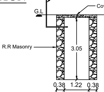
SOAKPIT SECTION
