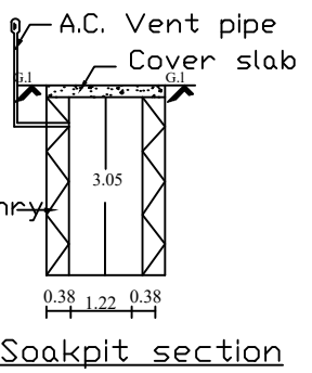
Soakpit section
