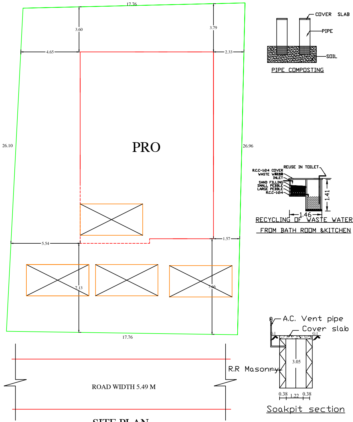
SITE PLAN
