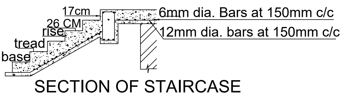
SECTION OF STAIRCASE
