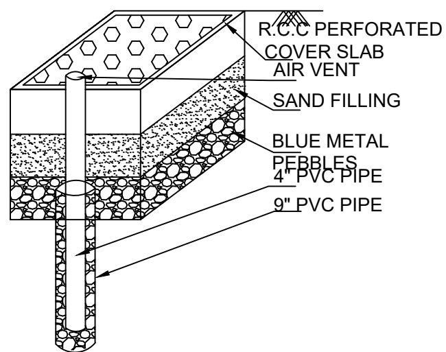
PERCOLATION BORE PIT
