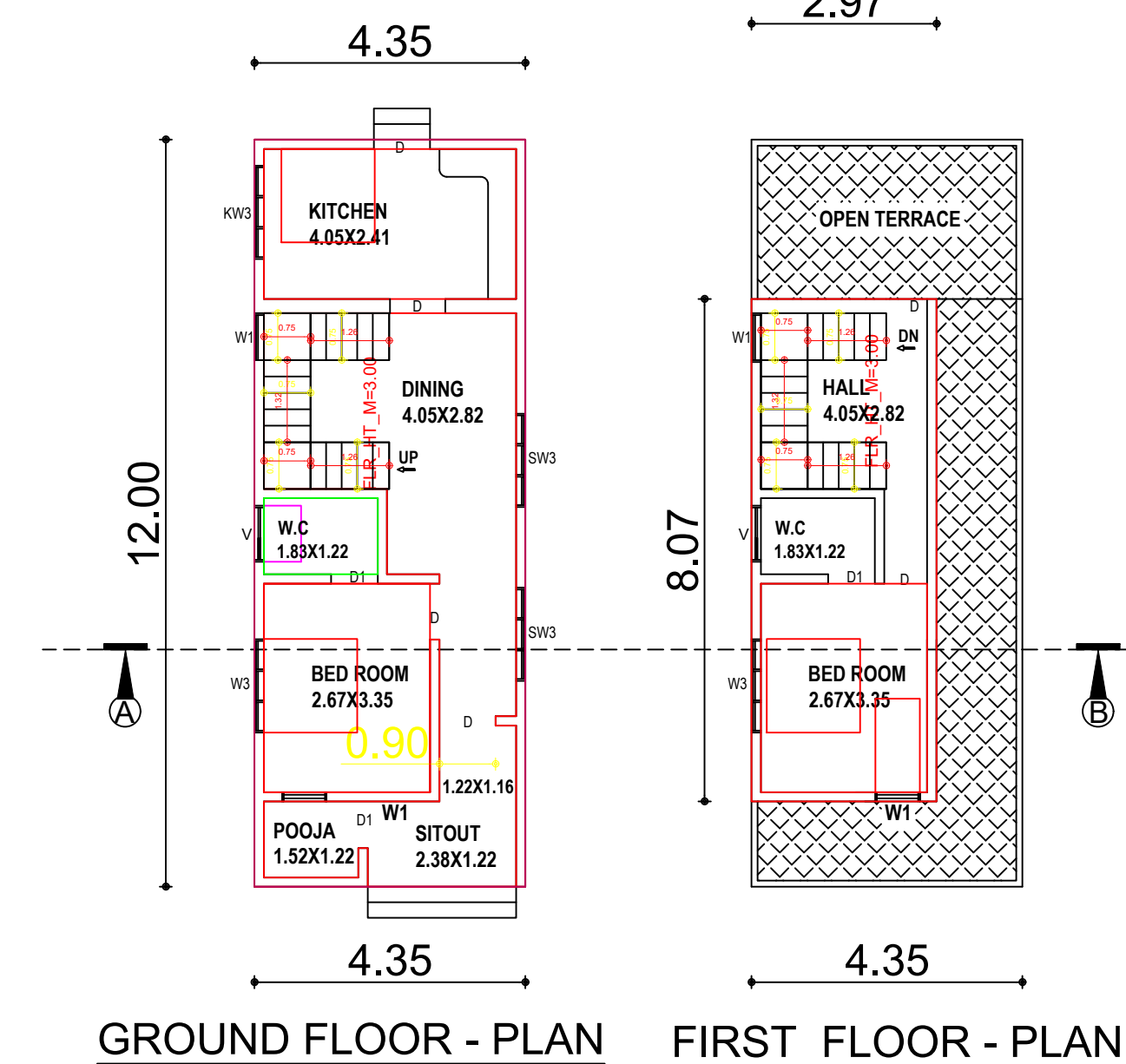
SCALE 1:100 ALL DIMENSIONS ARE IN METRE
