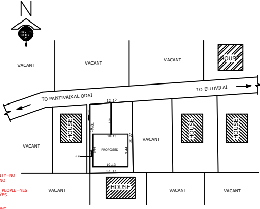
KEY PLAN [SCALE 1:400]
