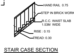
STAIR CASE SECTION
