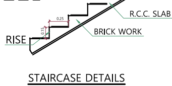
STAIRCASE DETAILS
