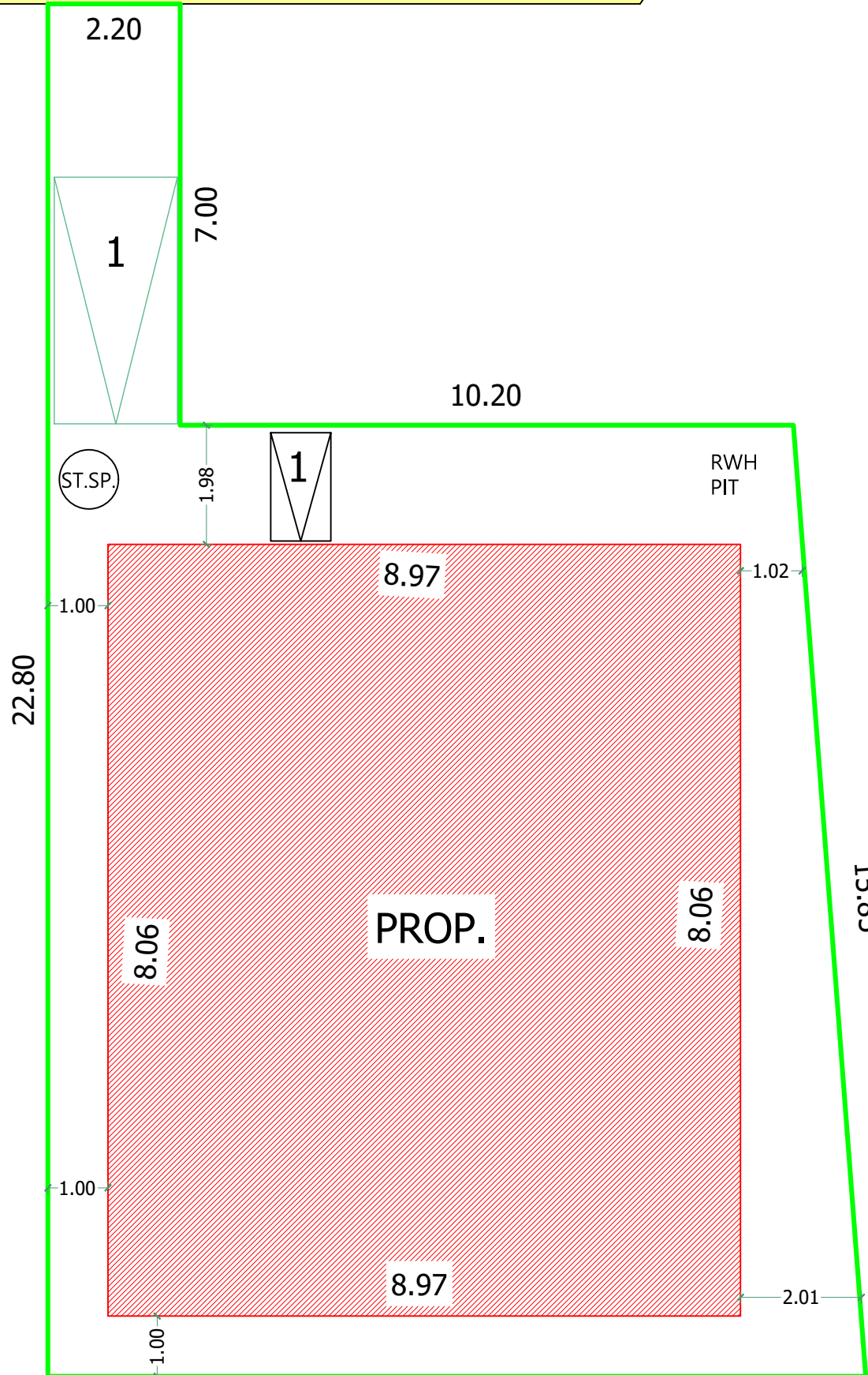
SITE PLAN
