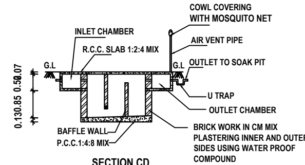
SECTION CD
