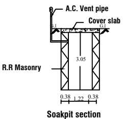
Soakpit section
