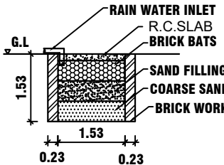
RAIN WATER NG PIT
