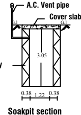
Soakpit section
