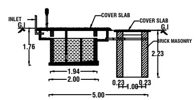
SECTION OF SEPTIC TANK
