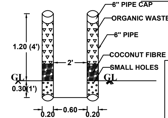
PIPE COMPOST PIT
