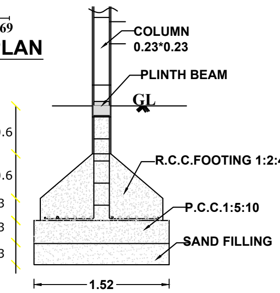
COLUMN DETAILS DETAIL "A"
