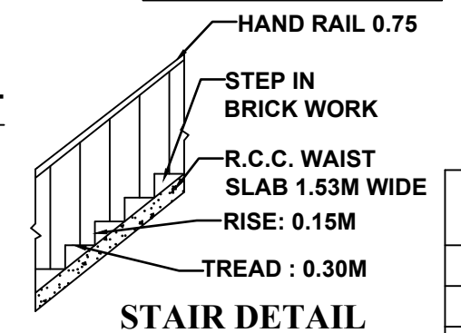
STAIR DETAIL
