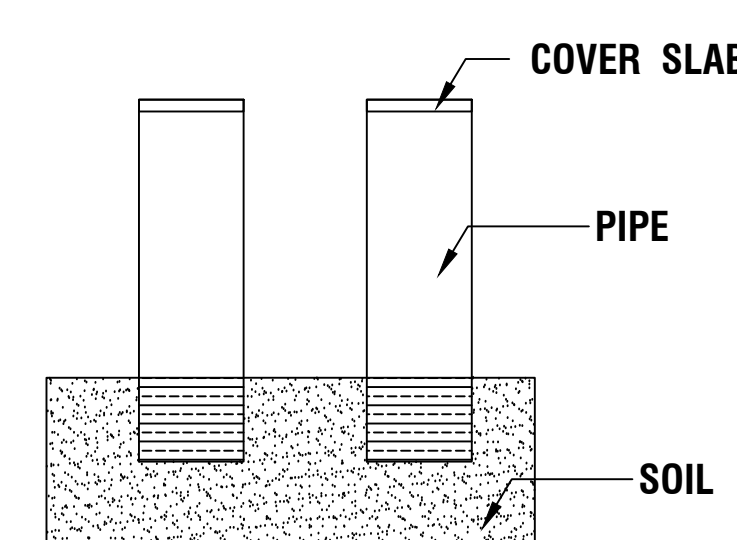
PIPE COMPOSTING
