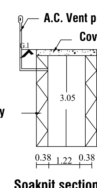
Soakpit section
