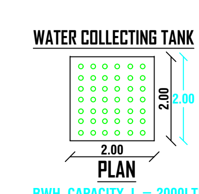
WATER COLLECTING TANK PLAN
