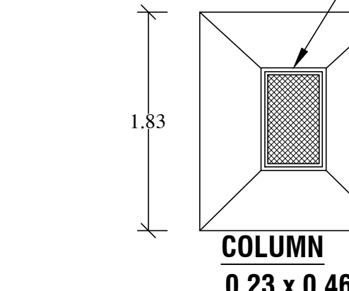
SECTION OF COLUMN
