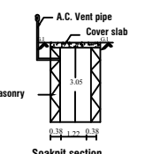
Soakpit section
