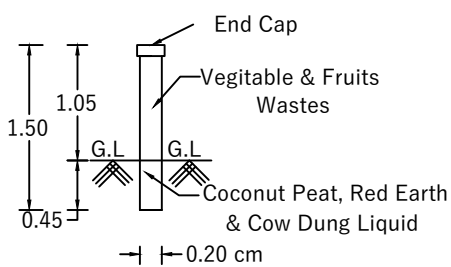
PIPE COMPOSTER
