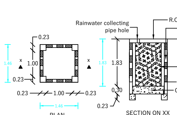
RAIN WATER HARVEST WELL
