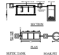
SEPTIC TANK
