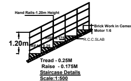
Staircase Details Scale:1:500
