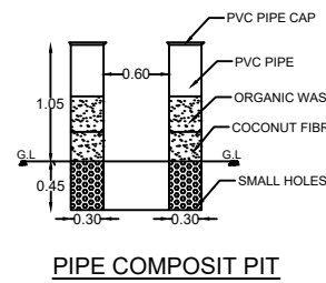
PIPE COMPOSIT PIT
