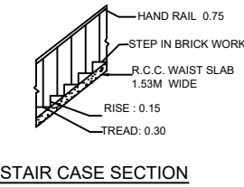
STAIR CASE SECTION
