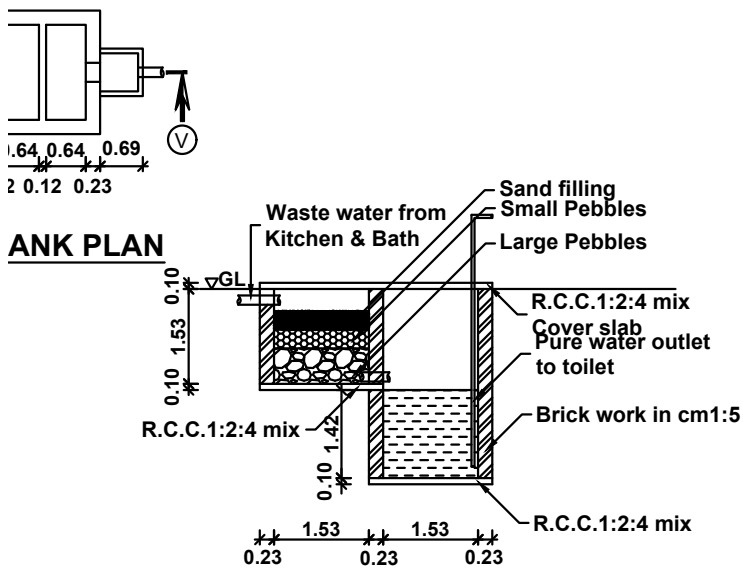
WASTE WATER RECYCLING SYSTEM
