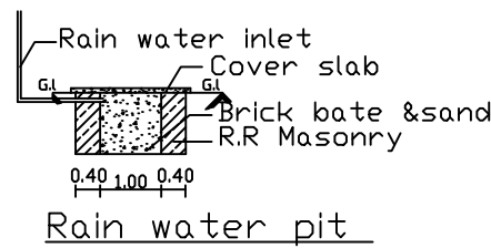
Rain water pit
