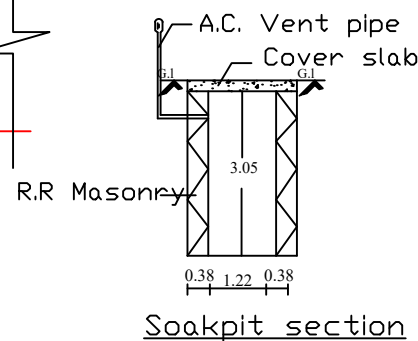
Soakpit section
