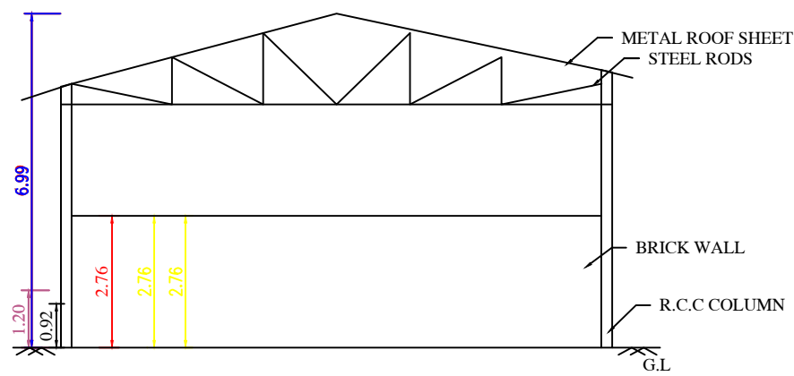
SECTION @ X-X'
