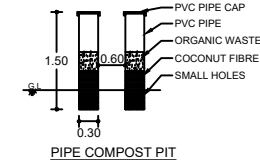
PIPE COMPOST PIT
