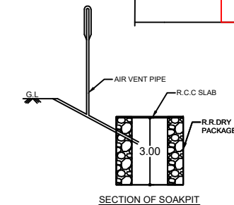
SECTION OF SOAKPIT
