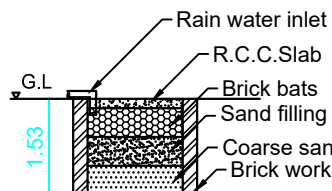
RAIN WATER
