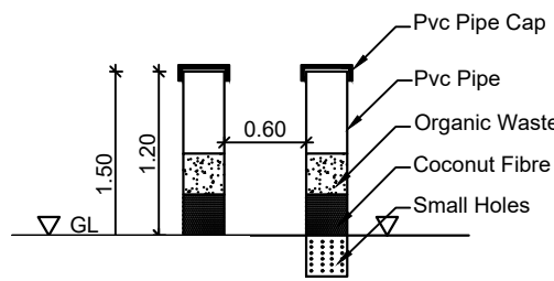
COMPOST PIT
