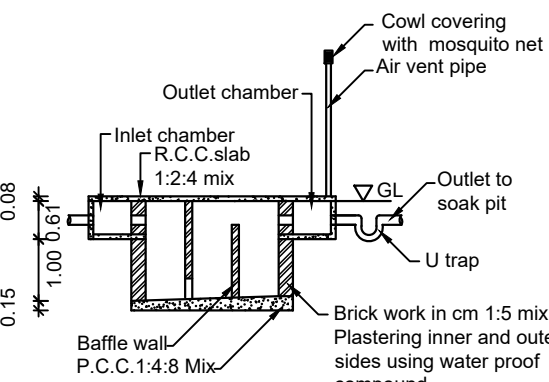
SECTION UV
