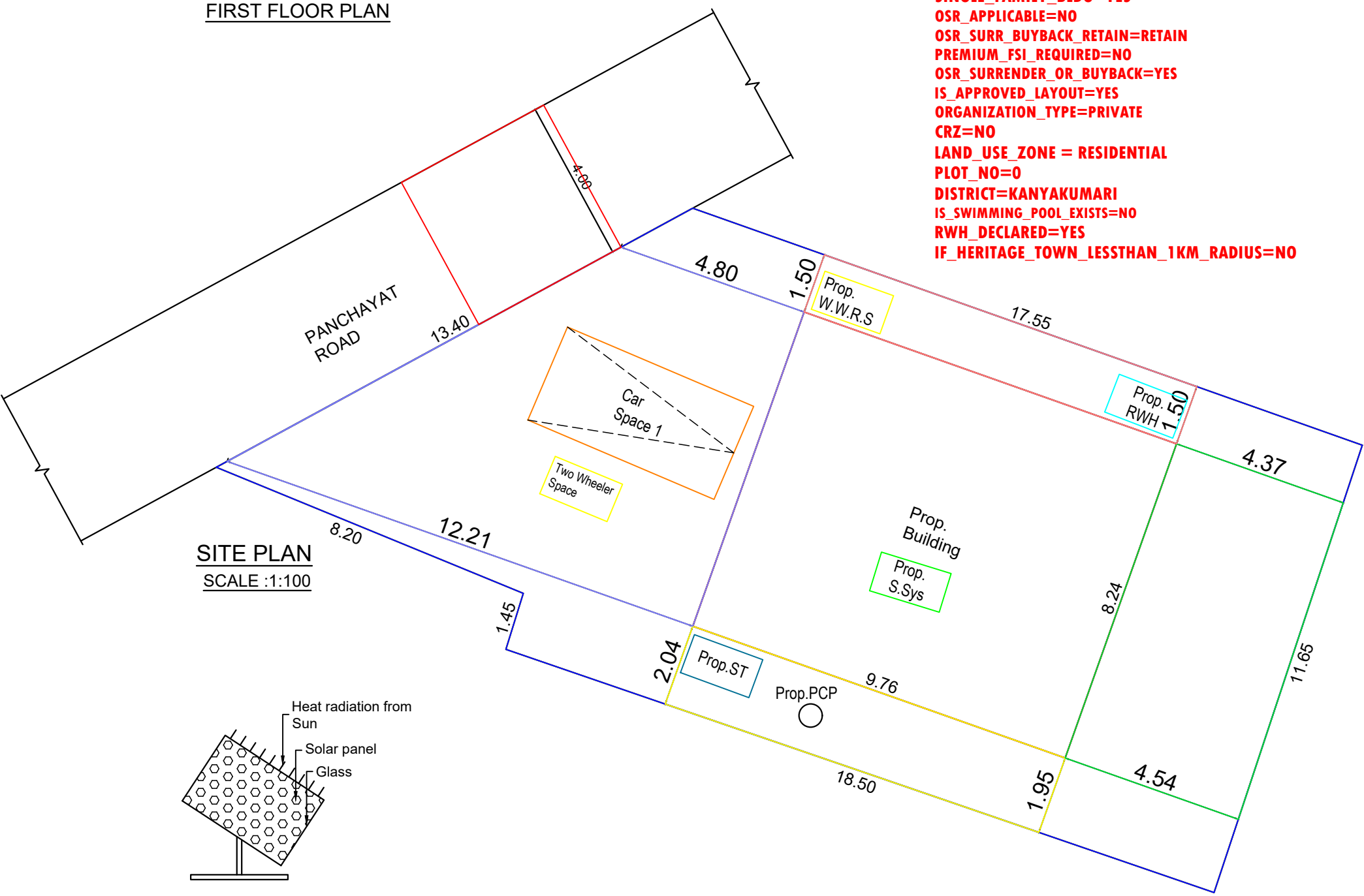
SOLAR SYSTEM
