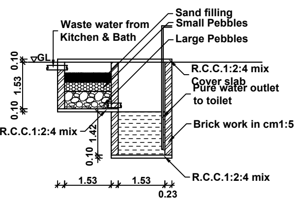
RECYCLING SYSTEM
