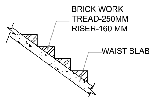
STAIRCASE DETAILS
