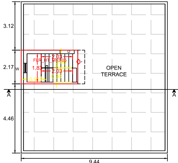
TERRACE PLAN
