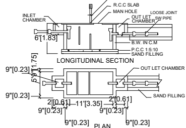
SEPTIC TANK:
