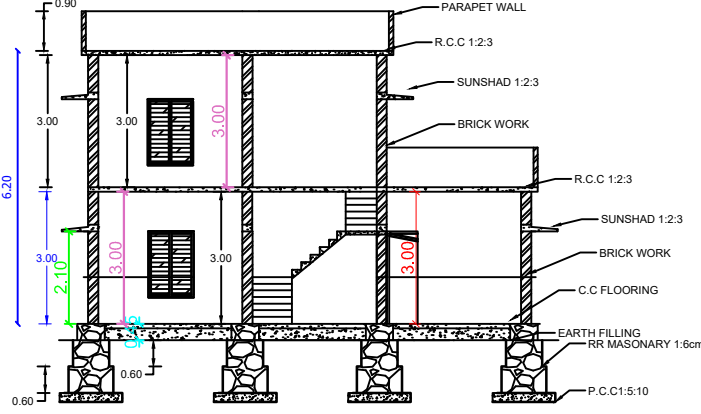
SECTION "A-B"
