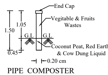
PIPE COMPOSTER
