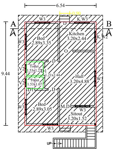
EXISTING GROUND FLOOR PLAN EXG. D.No: 21-11/5
