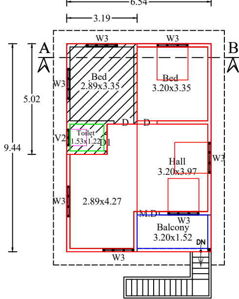
EXTENSION FIRST FLOOR PLAN
