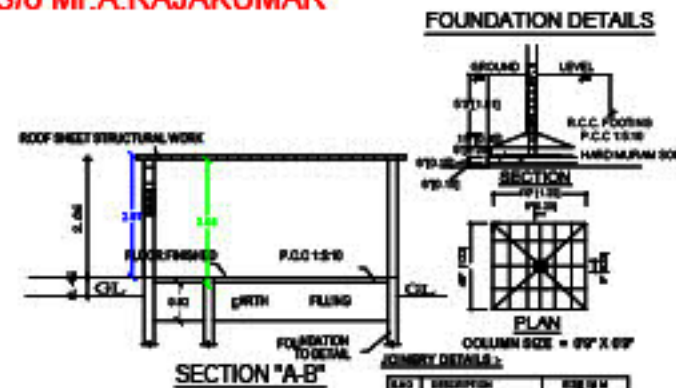
FOUNDATION DETAILS
