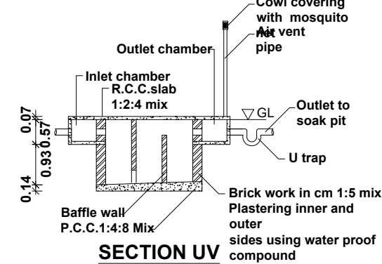
SECTION UV
