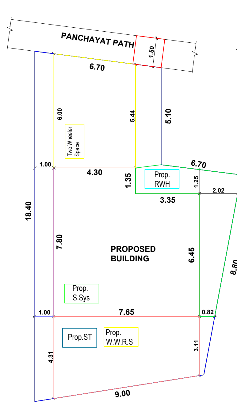
SITE PLAN
