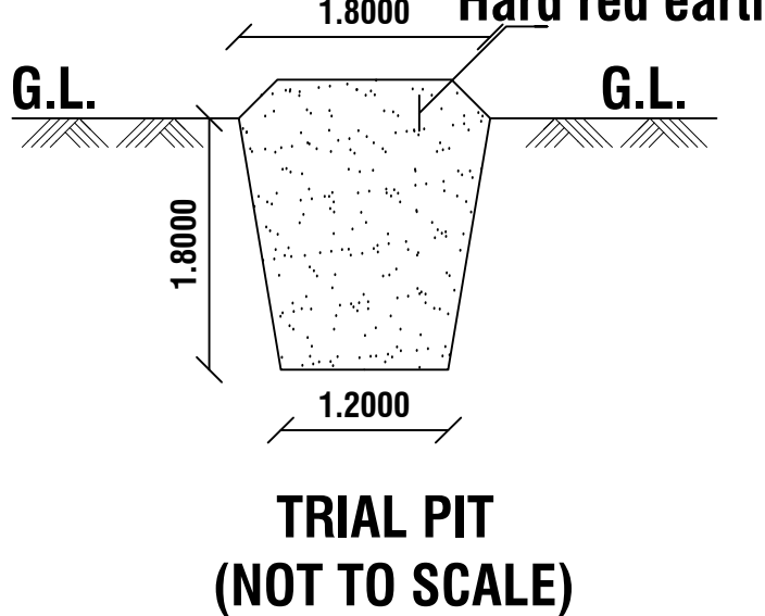
TRIAL PIT (NOT TO SCALE)
