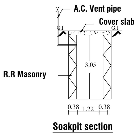
Soakpit section
