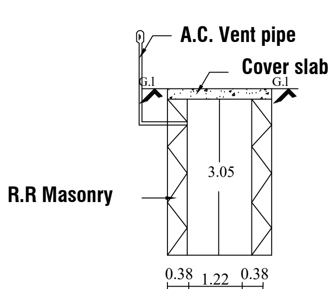
Soakpit section
