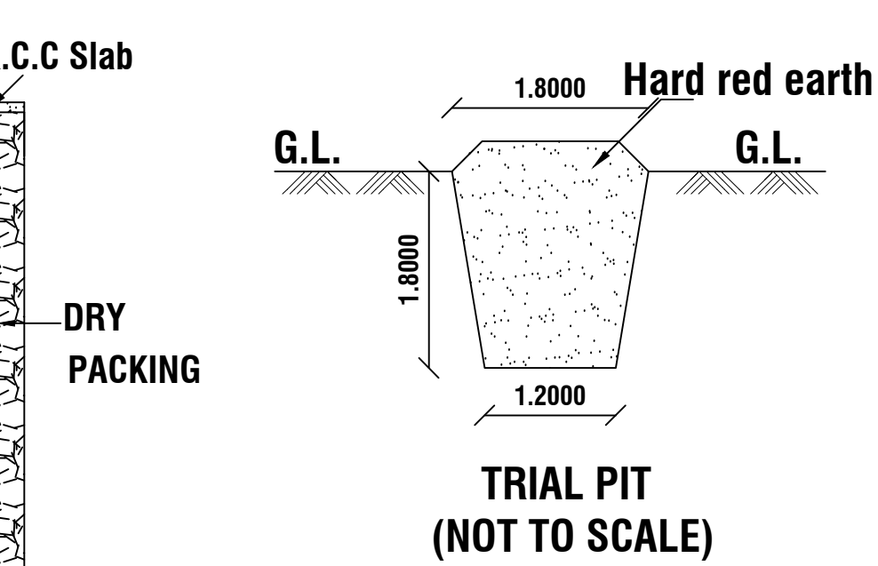
TRIAL PIT (NOT TO SCALE)
