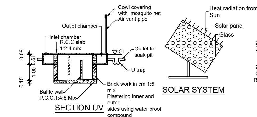
WASTE WATER RECYCLING SYSTEM
