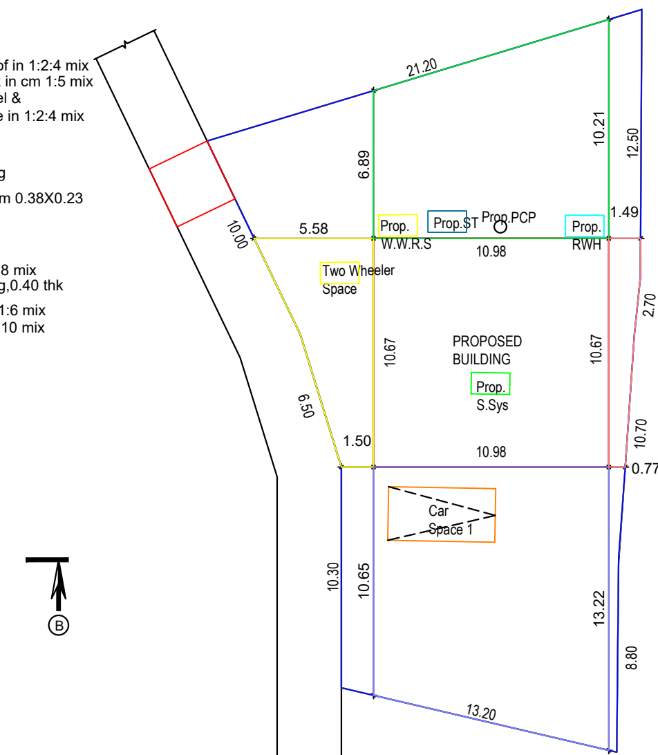
SITE PLAN
