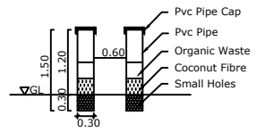
PIPE COMPOST PIT
