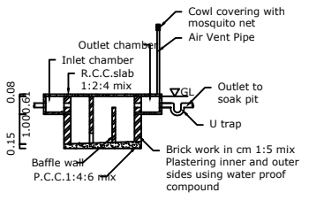
SECTION UV
