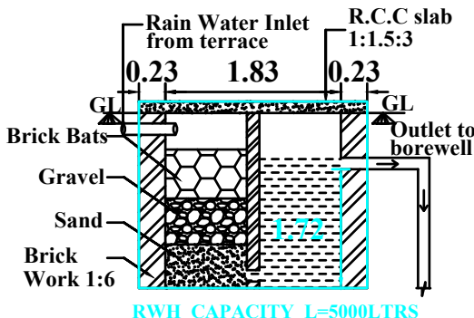
RAIN WATER HARVESTING - PIT
