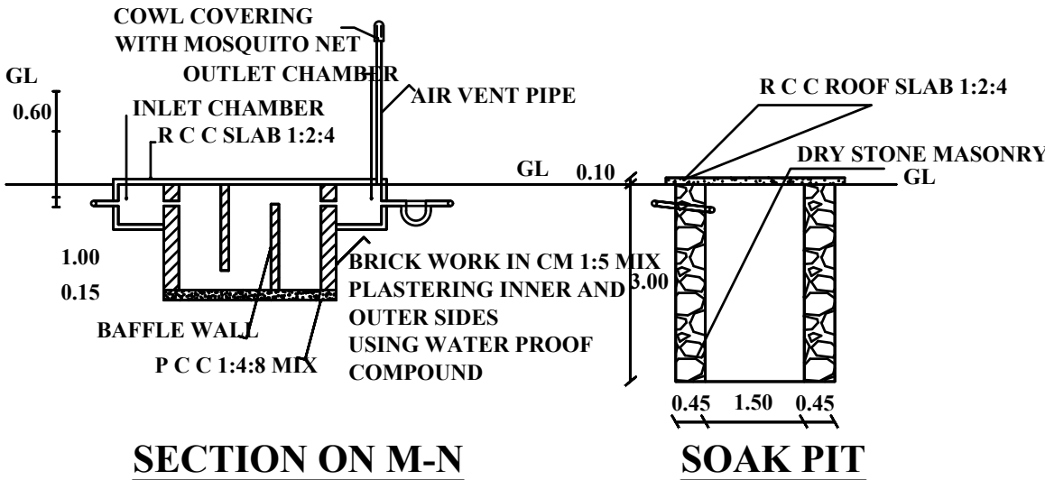
SECTION ON M-N
