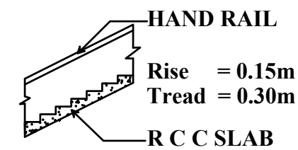
DETAILS OF STAIR CASE
