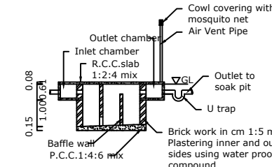
SECTION UV
