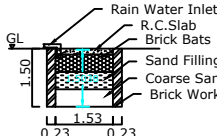
RAIN WATER HARVESTING PIT
