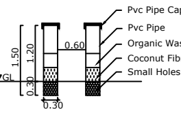
PIPE COMPOST PIT
