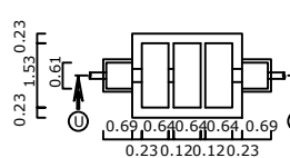
SEPTIC TANK PLAN
