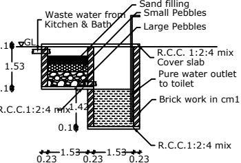
WASTE WATER RECYCLING SYSTEM
