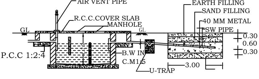
SECTION OF DISPERSION TRENCH
