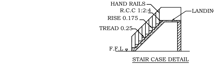
STAIR CASE DETAIL
