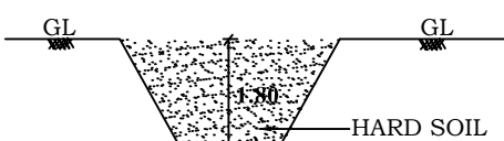
TRIAL PIT
