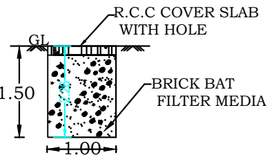
RAIN WATER HARVESTING PIT RWH_CAPACITY_L=5000LTRS
