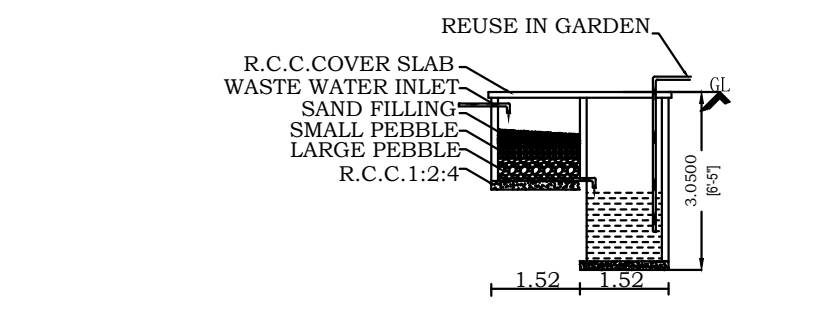
RECYCLING OF WASTE WATER
