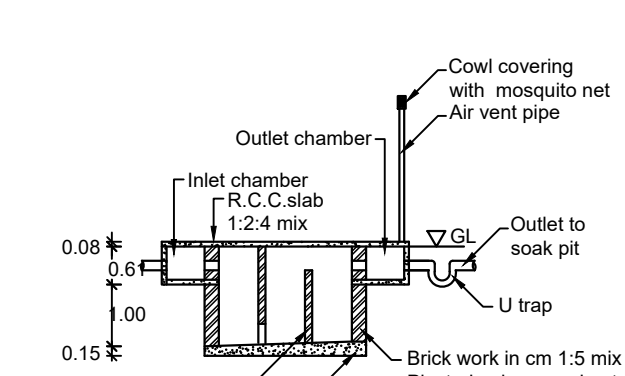
SECTION UV
