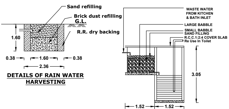
RECYCLING OF WASTE WATER FROM KITCHEN & BATHROOM
