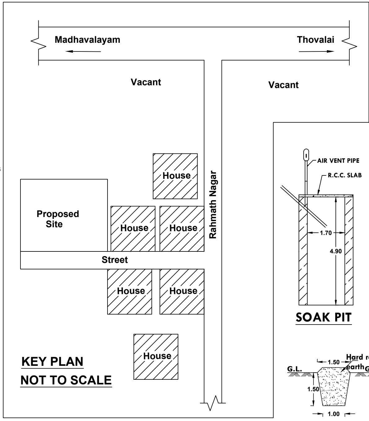
SOAK PIT (Scale 1:100)
