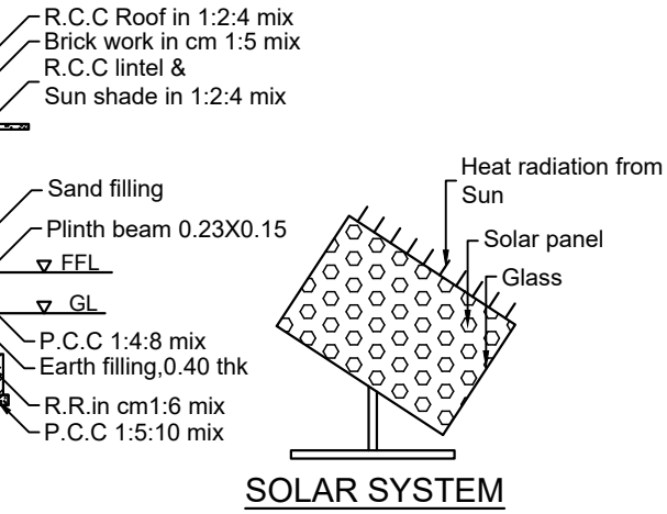
SOLAR SYSTEM
