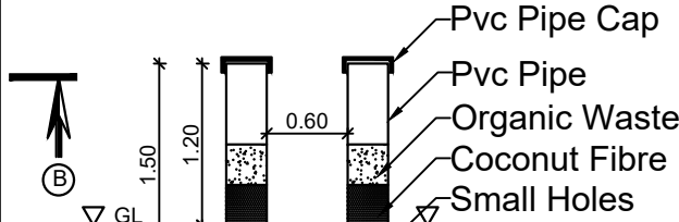
PIPE COMPOST PIT
